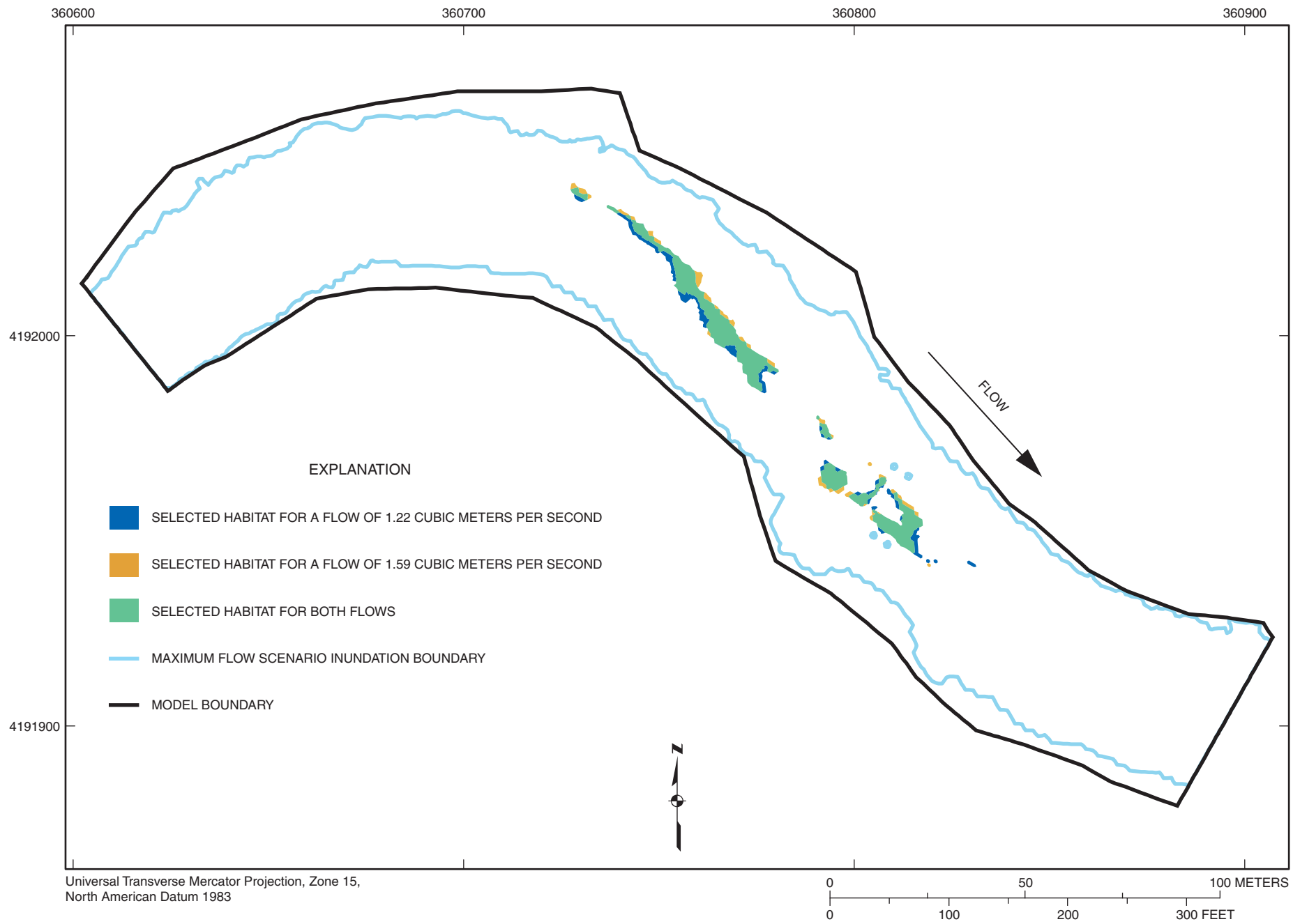
Figure 1-32. Selected habitat area distribution for habitat category 14 (flathead catfish) at flows of 1.22 and 1.59 cubic meters per second at Marmaton River site M1.
